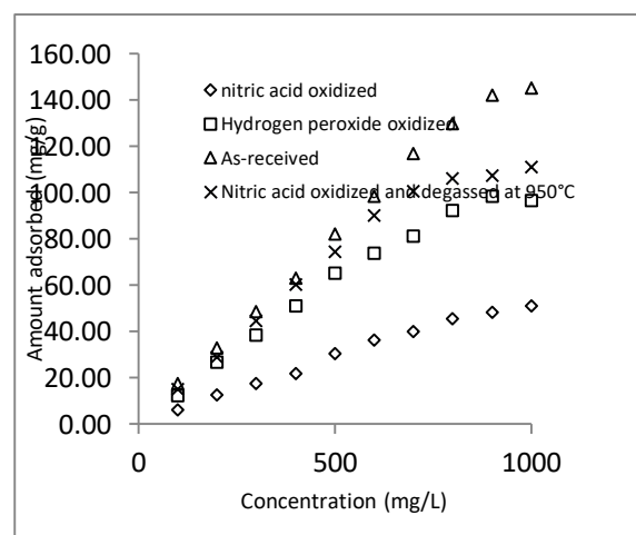
Fig.4. Adsorption isotherms of tartrazine for as-received, oxidized and degassed ACs
