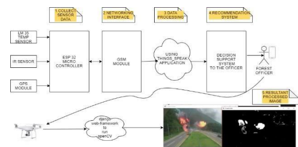
Fig. 3. System Architecture
