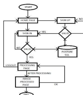
Fig. 4. Flowchart of Django web-app for processing
