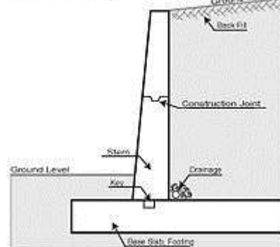
Fig 1. Cantilever Retaining Wall
