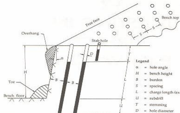
Fig 2. Surface Blasting Terminologies.
