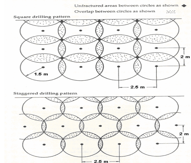
Fig 3: Square versus staggered pattern. Optimum coverage is achieved in staggered pattern.
