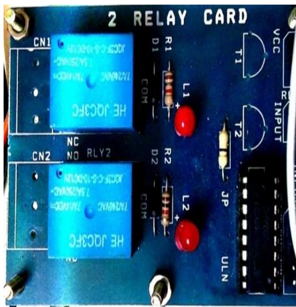
Fig. 5. Two Relay Board
