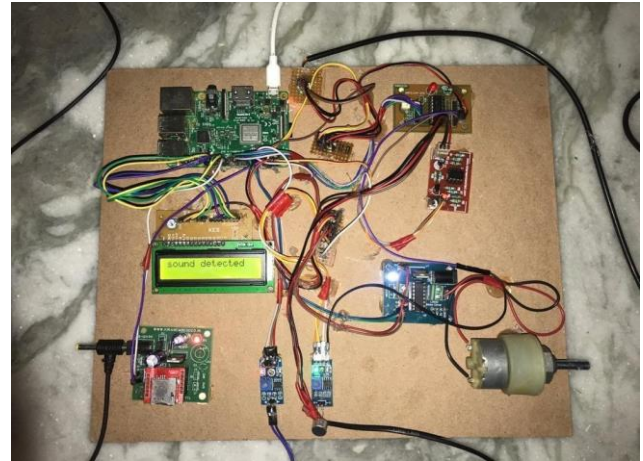
Fig.5(e) Baby Cry Detection
