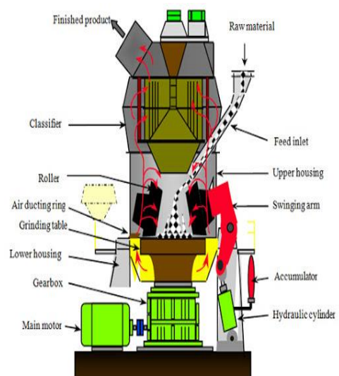
Fig. 2. Vertical Cement Mill
