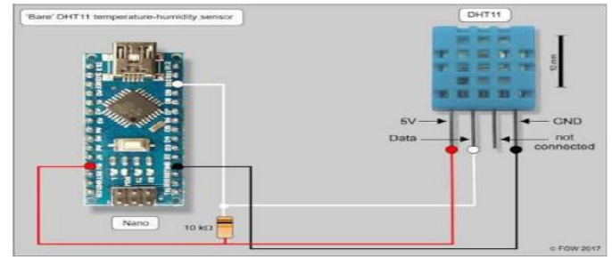
Fig. 1.DHT11 PIN CONFIGURATION [9]
