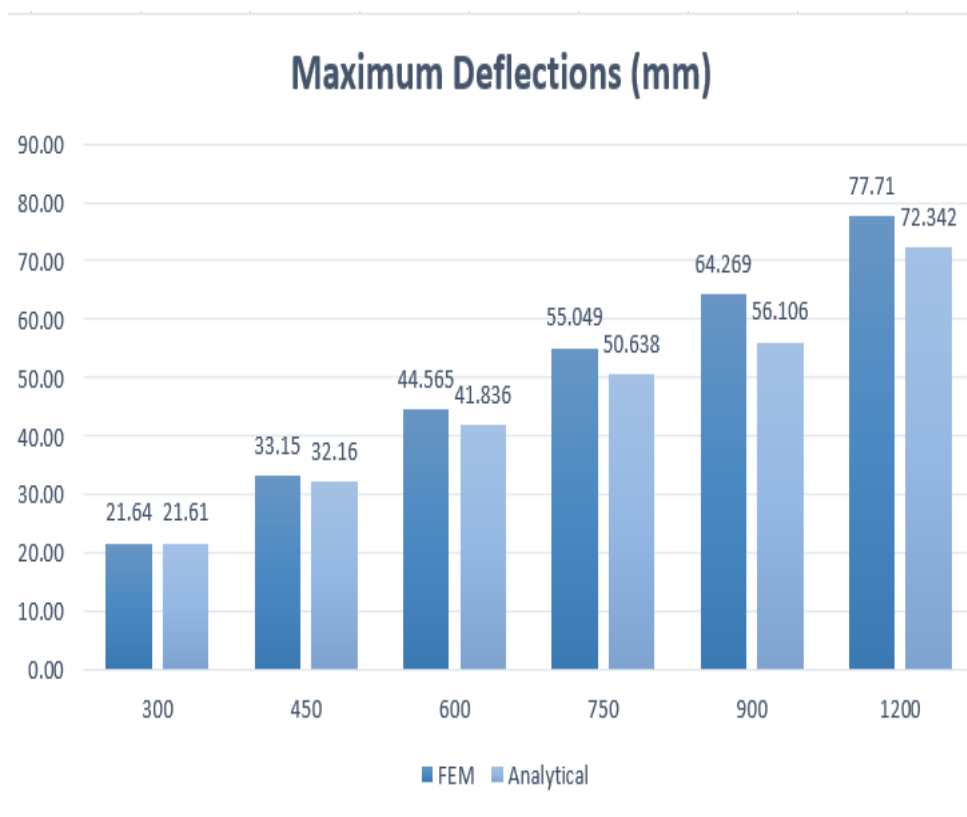
Chart 11. Maximum deflection comparison FEM and Analytical values
