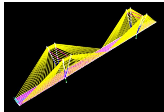
Model (4) – Pylon inclined at 15°
