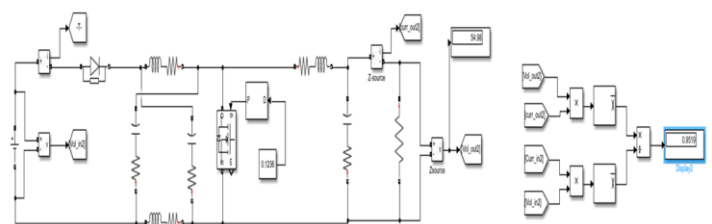
Fig. 5. Z-source Converter
