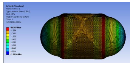
Contour plot for GFRP cylinder hoop stress
