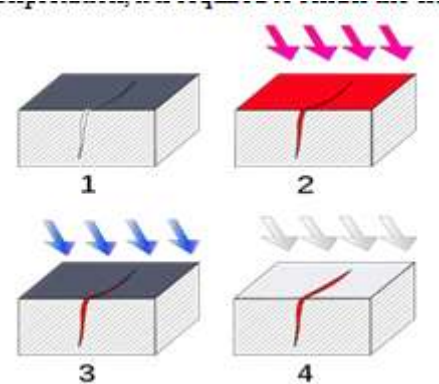
Fig. 2. Each step of Liquid Penetrant Testing
