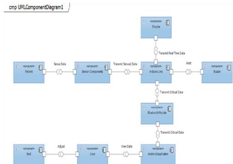
Figure 3 - Component diagram
