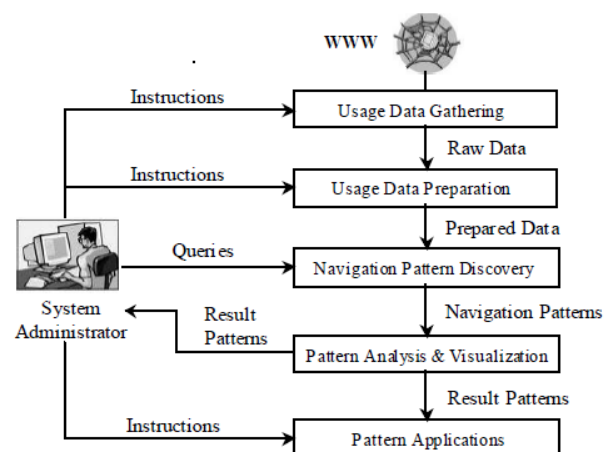
Fig. 2. Web Usage Mining System Structure
