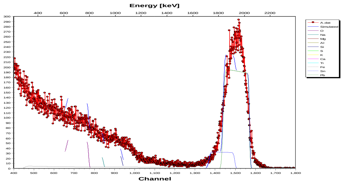
Figure 3.1. The Rutherford backscattering spectrometry (RBS) for sample A.
