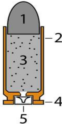
Fig (2) cartridge components [1]
