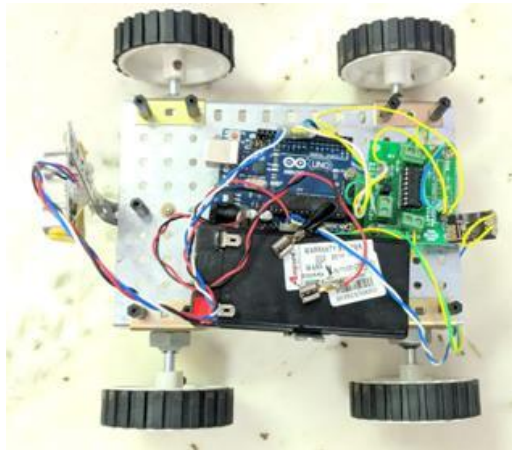
Fig. 9. Top View
