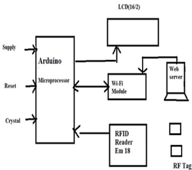
Figure 7.1 System Architecture
