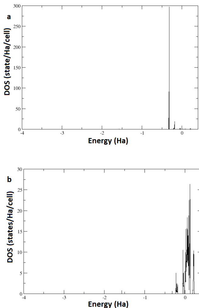
Figure 8: The partial density of states for the S atoms in AgGaS 2 . (a) The S-3s partial-DOS (b) S-3p partial DOS
