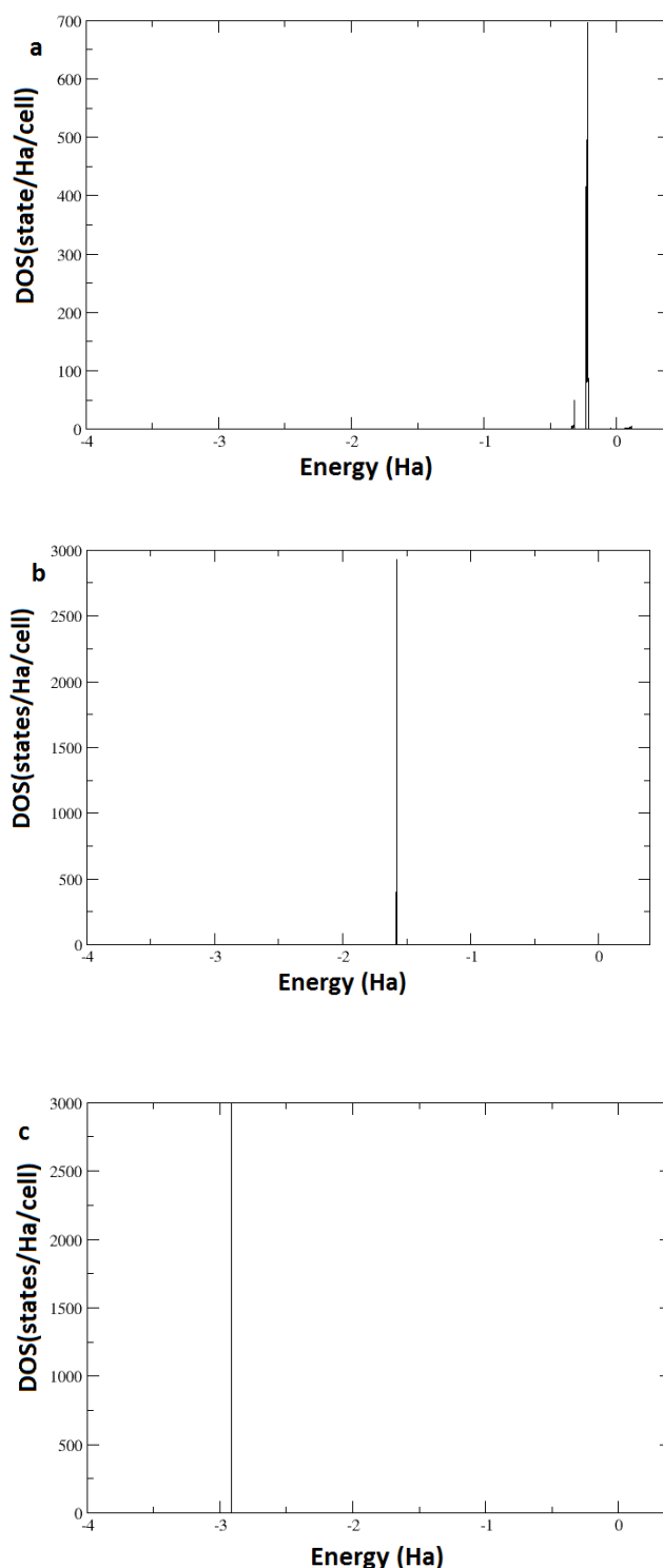
Figure 9: The partial density of states for the Ag atoms in AgGaSe 2 . (a) Ag-4d partial-DOS (b) Ag-4p partial DOS (c) Ag-4s and Ag-5s partial DOS.
