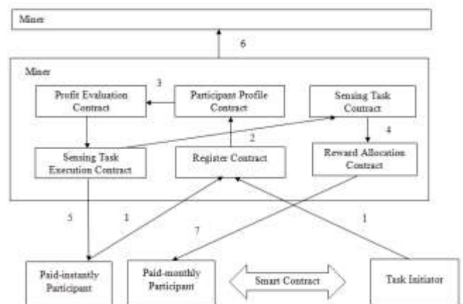
Figure 3. Workflow of the blockchain-based MCS.
