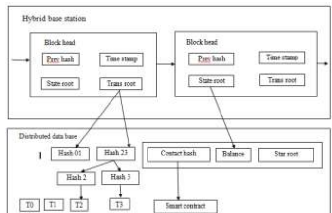
Figure 2. Structure of block in the blockchain-based MCS.
