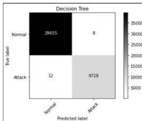
Fig. 8. RF confusion matrix (Network)
