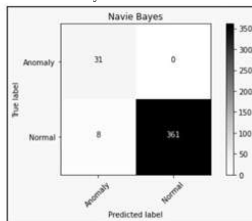
Fig. 7. MNB confusion matrix (BGL)
