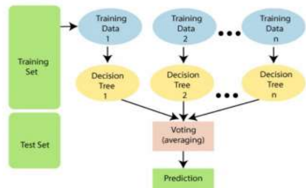
Fig. 2. Random Forest
