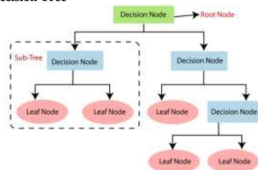
Fig. 3. Decision tree
