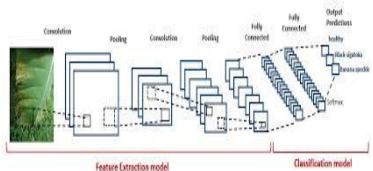
Fig 8: Working of CNN
