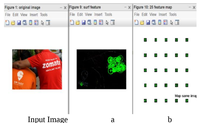
Fig.5 SURF feature
