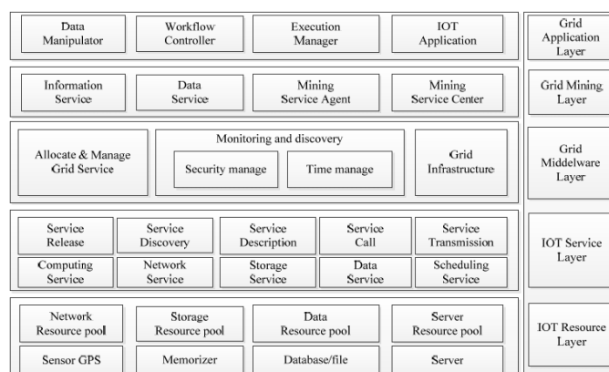
Fig.5 Grid based Data mining Model
