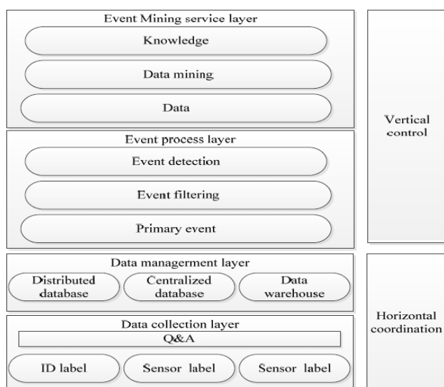
Fig.3 Multilayer Data Mining Model for IoT
