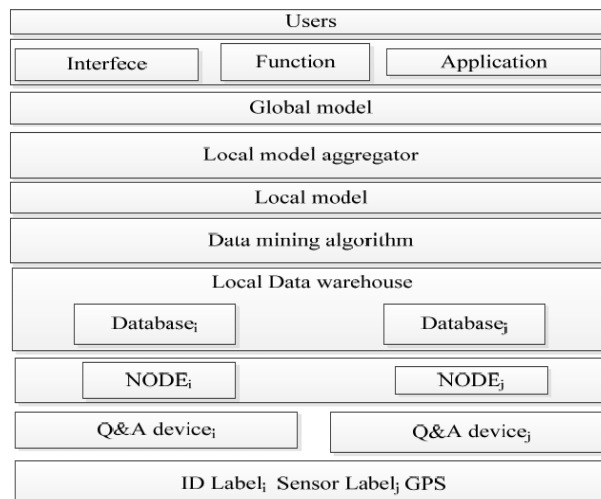
Fig.4 Data mining model for distributed architecture
