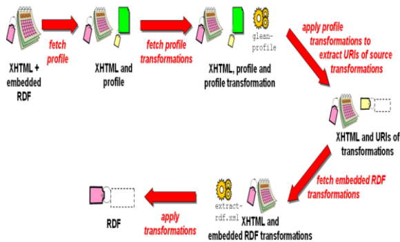
Fig. 3. Sequence of RDF documents with profile construction.
