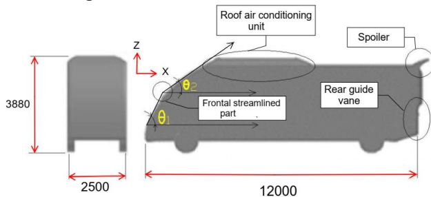
Figure.3: Streamline design concept used.
