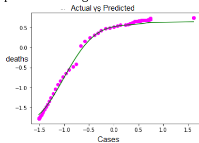
Fig.3. Actual vs Predicted deaths in China using SVR
