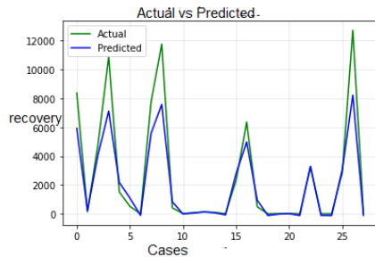
Fig. 19. Actual vs Predicted recovery in India using DL
