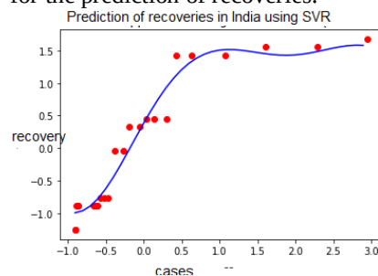
Fig. 16. Actual vs Predicted recovery in India using SVR
