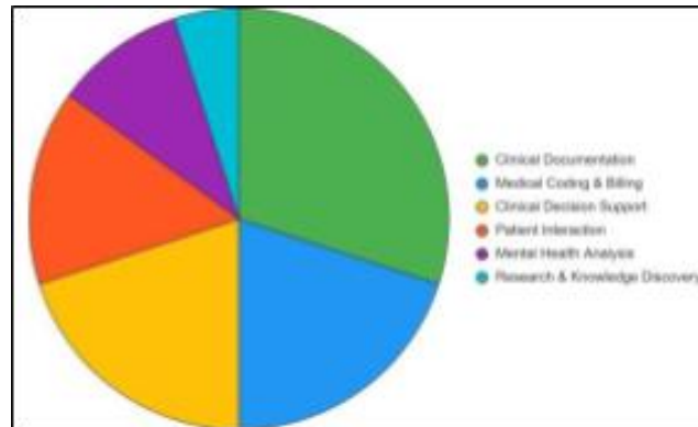
Figure 2. NLP applications
