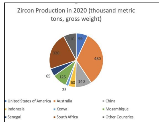
Fig. 1. Zircon Production in 2020 (usgs)
