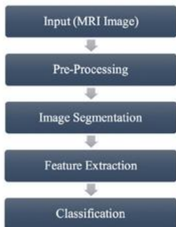
Fig 1. methodology
