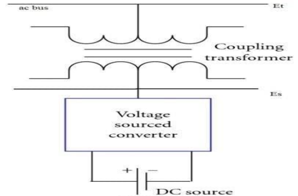
STATIC SYNCHRONOUS COMPENSATOR.
