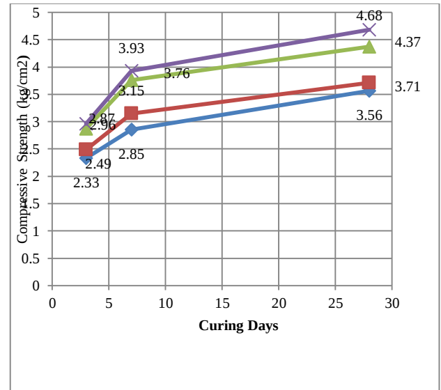
Fig. 3 UCS value at (5% - 20% of SDA) with varying combinations of Soil and ESP
