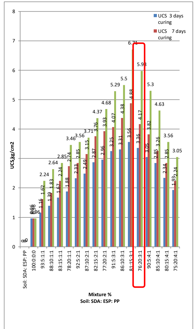
Fig. 1 Variation of Unconfined Compressive Strength due to change in mix proportions.
