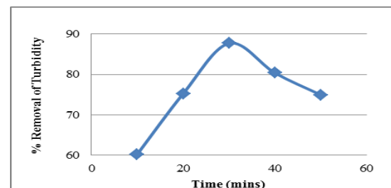
Fig. 8. Effect of contact time on turbidity removal using aloe vera
