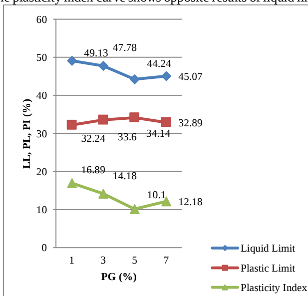
Fig.3.3 Consistency limits of mix having 20% FA And 1.5% HHF with various proportion of PG and Soil
