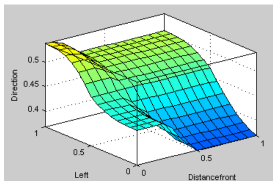
e- path 5
