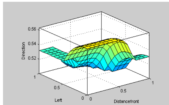
d- path 4
