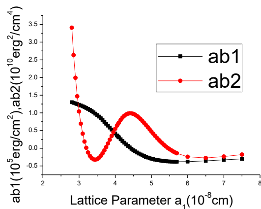
Figure 6 Variation of ab_1 and ab_2 with lattice parameter a_1 for Morse potential.
