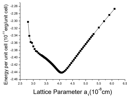
Figure 4 Variation of energy per unit cell (E) with lattice parameter a_1 .
