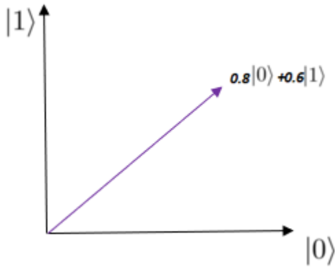
Fig. 1. Diagrammatical illustration of the vector nature of a qubit’s quantum state in the two-dimensional vector state space
