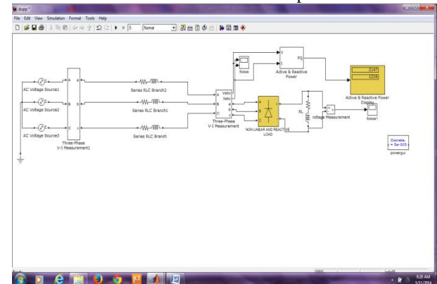
Fig 2. simulated diagram of nonlinear and reactive load
