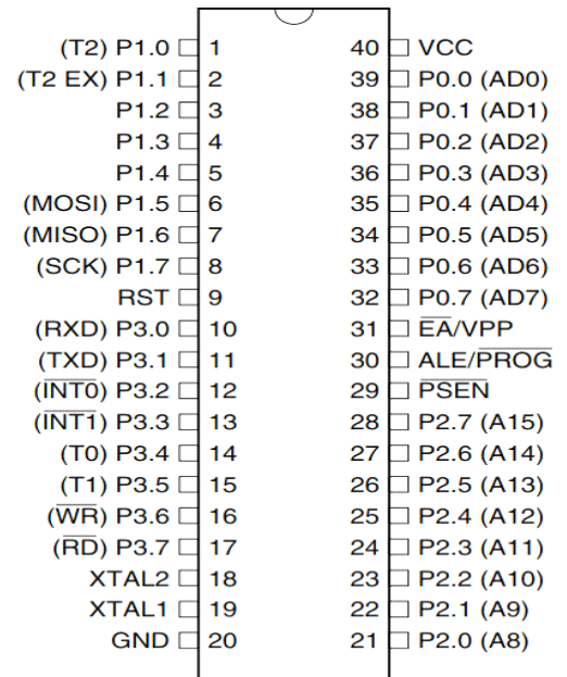
Fig .2 AT89S52 microcontroller
