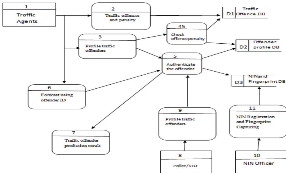
Figure 4: Data Flow Diagram of the proposed system
