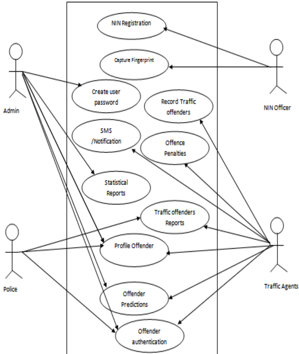
Figure 5: Use Case Diagram of the proposed system
