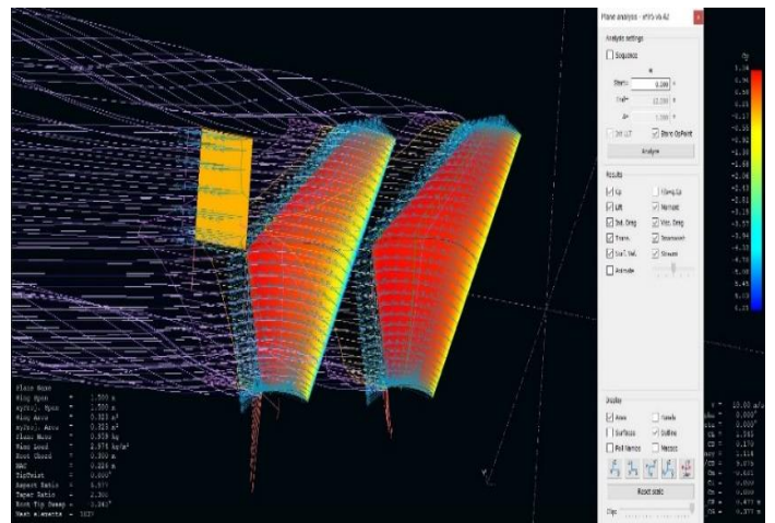
Figure 9: static pressure countour over airfoil The complete model fluid analysis is performed in xflr 5 . The analysis is performed at 10 m/s at 3 degree angle of attack.
