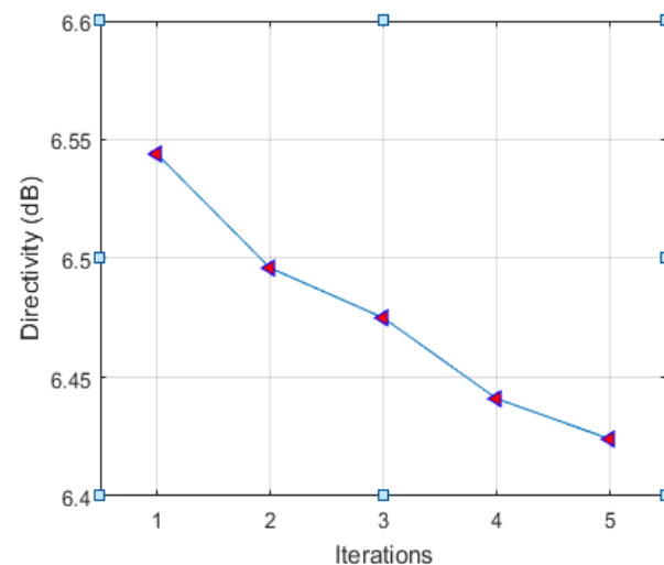
Fig. 8 Directivity
