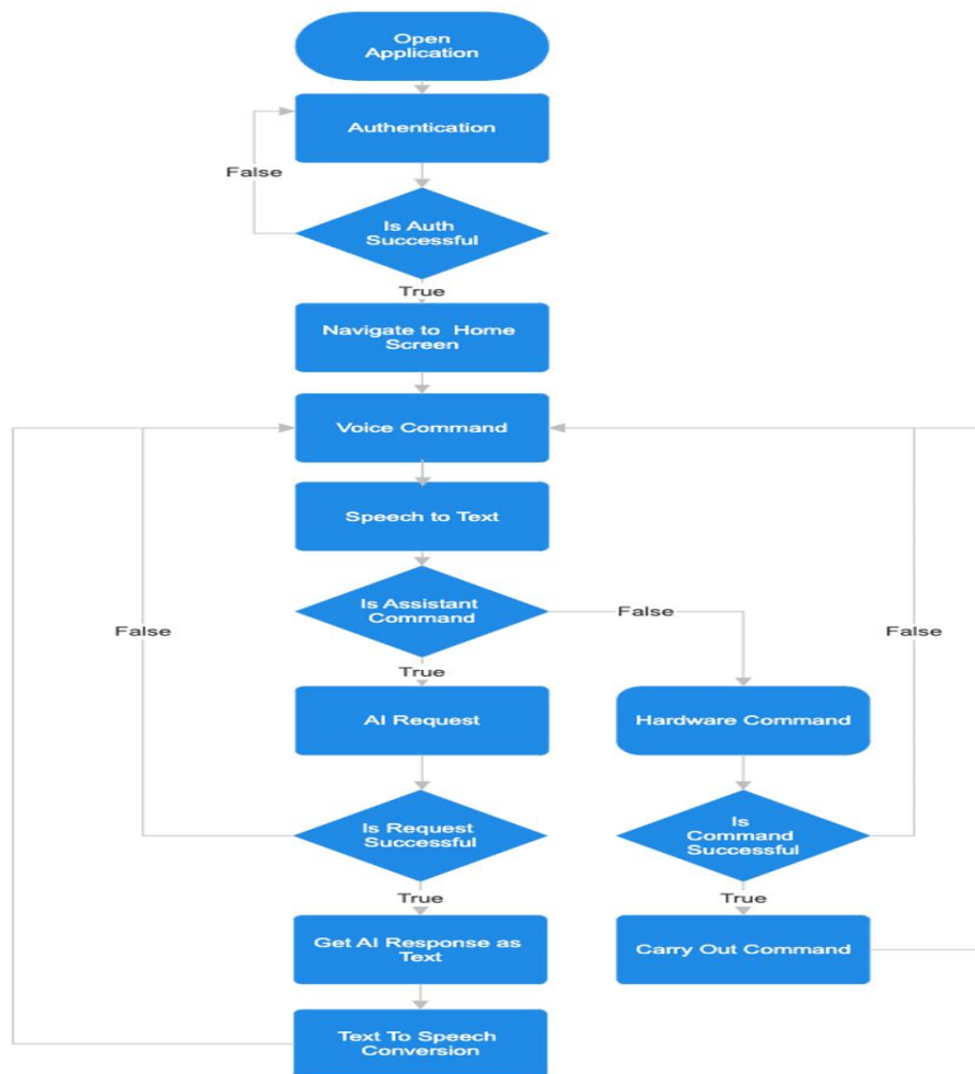
Fig. 1. System Flowchart
