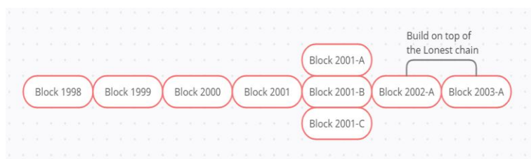
Figure 4: Building Chain Using Longest Chain Rule
