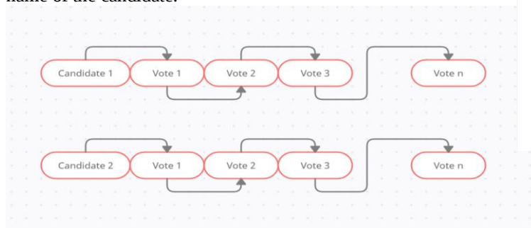
Figure 1: Creation of blockchains for each candidate
