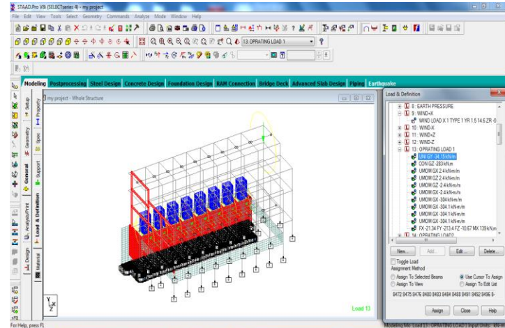
Fig7: operating load1
