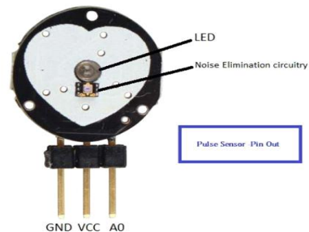
Figure 4 Pulse Sensor
