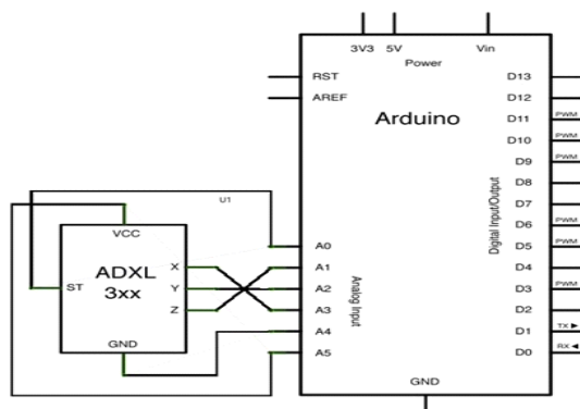
Figure 3 Interfacing ADXL with Arduino
