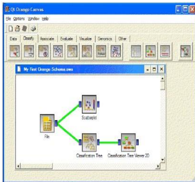
Figure 3: ORANGE GUI
