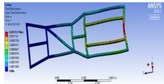
Figure 9. Result of rear impact
