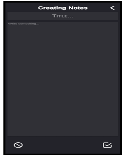
Figure 11. Note creation
