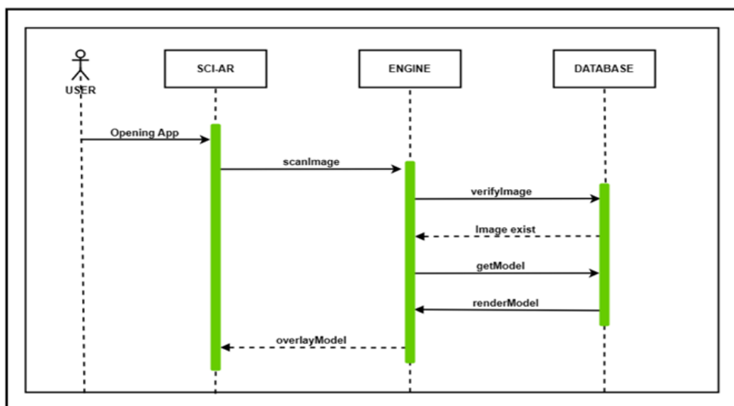
Figure 8. Sequence Diagram
