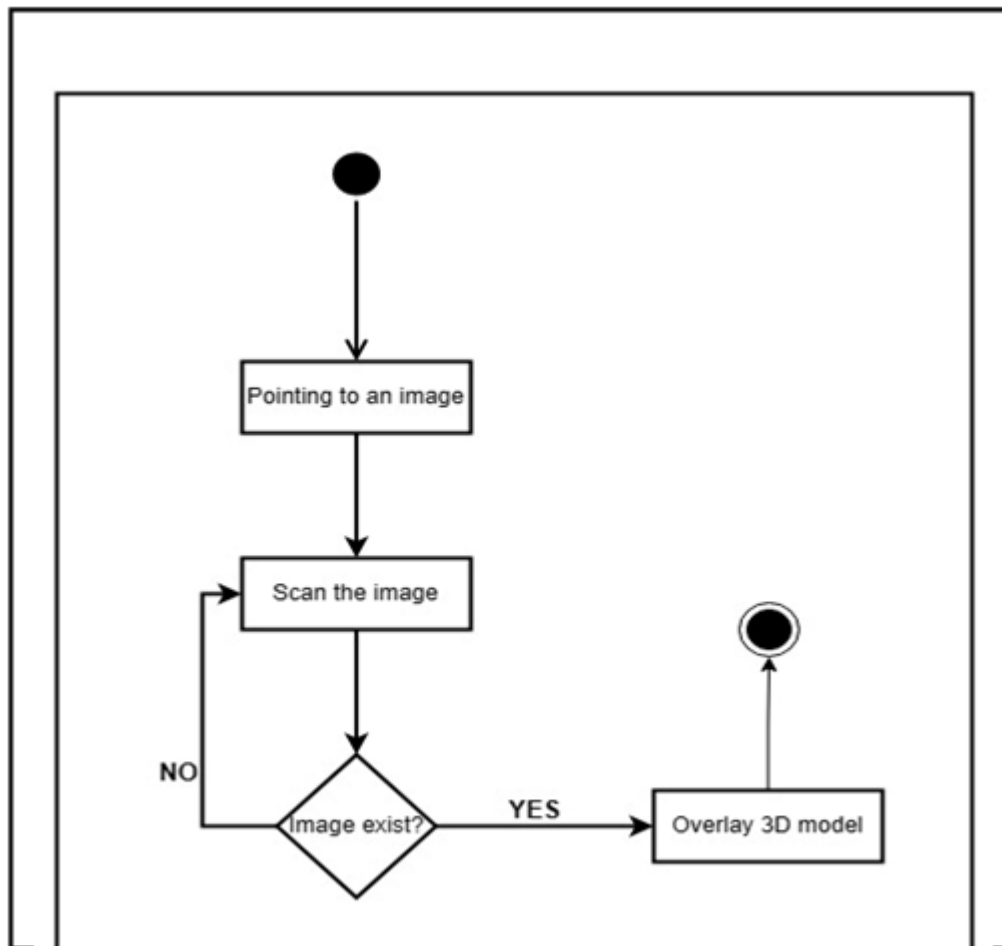
Figure 9. Activity Diagram
